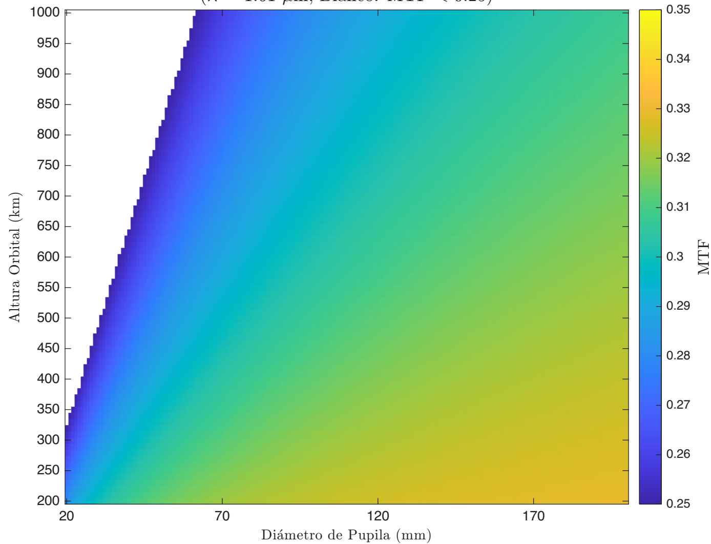
MTF - Korsch - Detector 2 ( \lambda = 1.61 \mu\text{m} , Blanco: MTF < 0.25)
